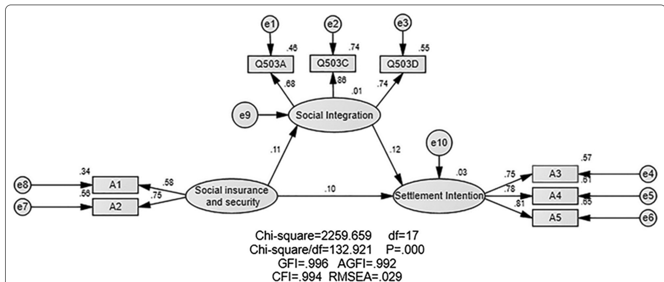
Fig. 1 Structural equation model Note. Rectangles and ovals represent observed and latent variables, respectively. e represents residual variance. AGFI: Adjust the Index of Good Fit. CFI: Comparative Fit Index. RMSEA: Root Mean Square Error of Approximation. p values < 0.01: significant correlation between variables. A1: BMIUE; A2: Apply for personal medical insurance cards; A3: Health education in occupational disease prevention; A4: Health education on prevention and treatment of chronic diseases; A5: Health education on STD and AIDS prevention; Q503A: Do you agree with the statement I like the city/place where I live now? Q503C: Do you agree with the statement that I would like to be a part of the local people? Q503D: Do you agree with the statement "I think the local people are willing to accept me as a member"?
